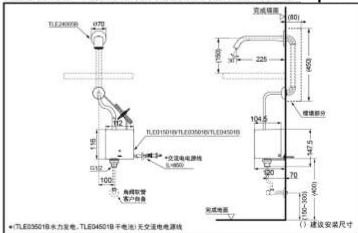
TOTO(CHINA) CO.,LTD. All rights reserved. TLE24005B+TLE01501B/TLE03501B/TLE04501B +TLE05701B Aqua-auto faucet(thermal)
