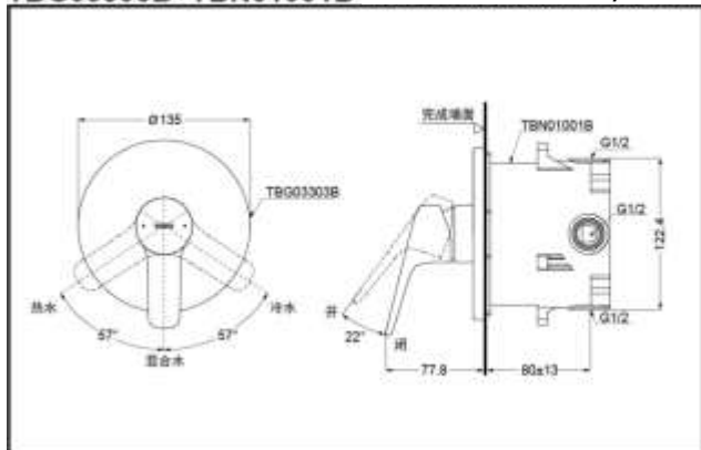
TBG03303B+TBN01001B Wall-Mount Mixer/Valve
